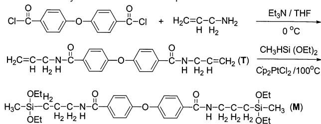
Scheme 1. Synthetic Route to Template T and Monomer M
