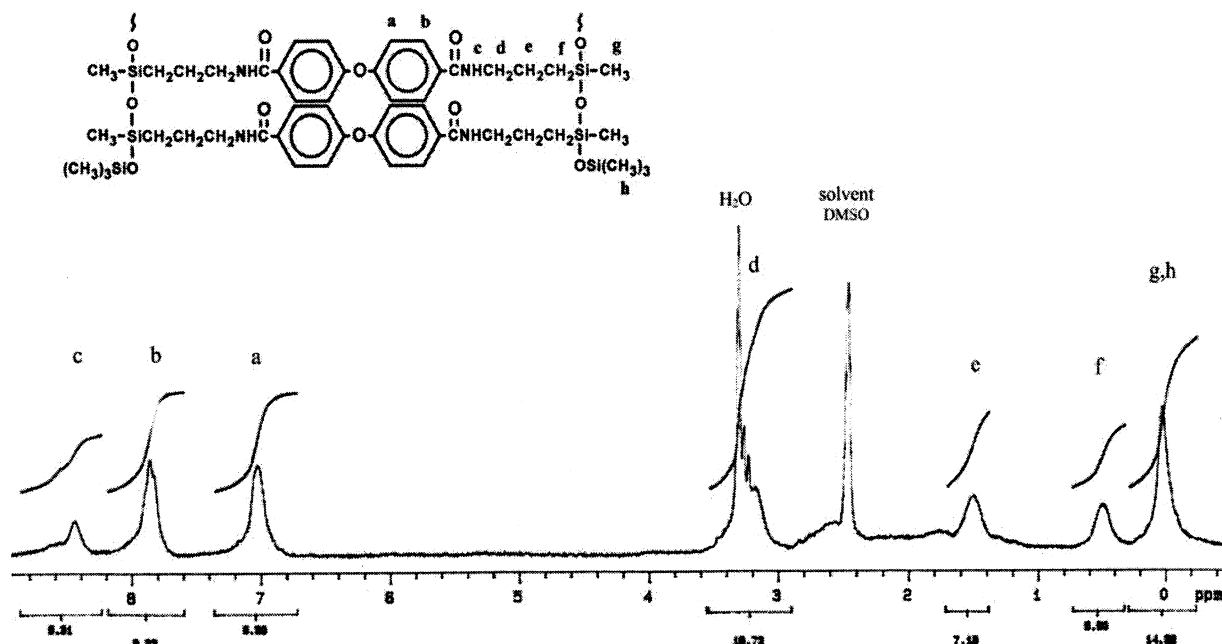
Figure 4. ^1\text{H} NMR spectrum of the polymer A-LPMS.
