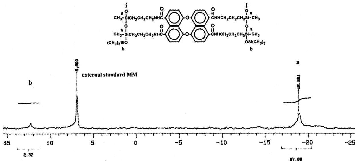
Figure 5. ^{29}\text{Si} NMR spectrum of the polymer A-LPMS.
