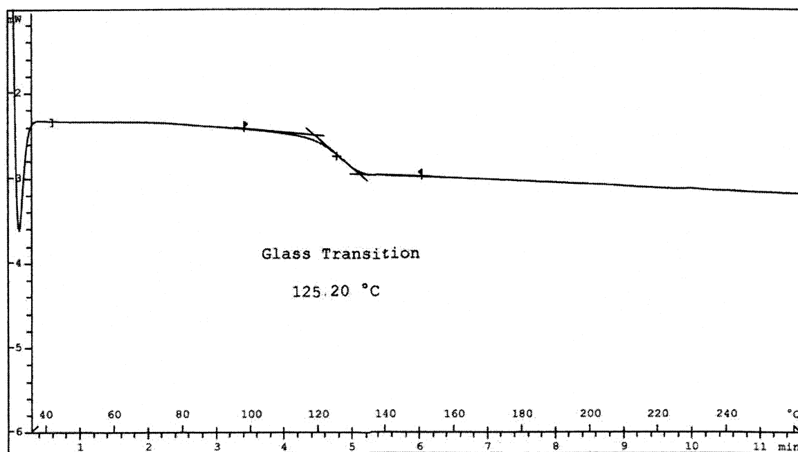
Figure 7. DSC curve of the polymer A-LPMS.
