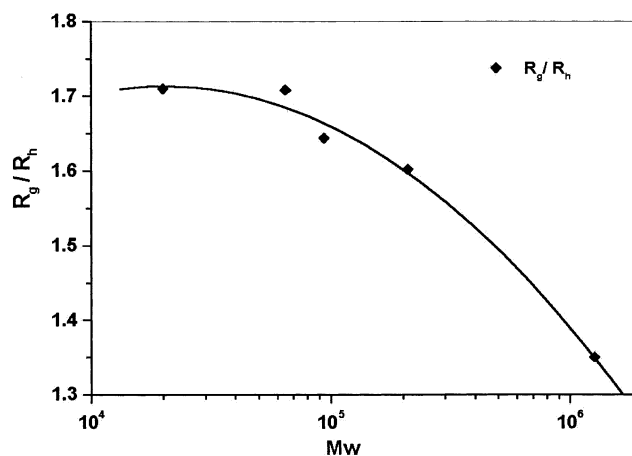
Figure 1. The relationship between R_g/R_h and M_w of the polymer A-LPMS.
