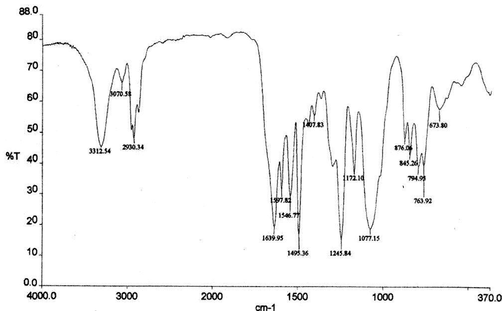
Figure 3. FTIR spectrum of the polymer A-LPMS.
