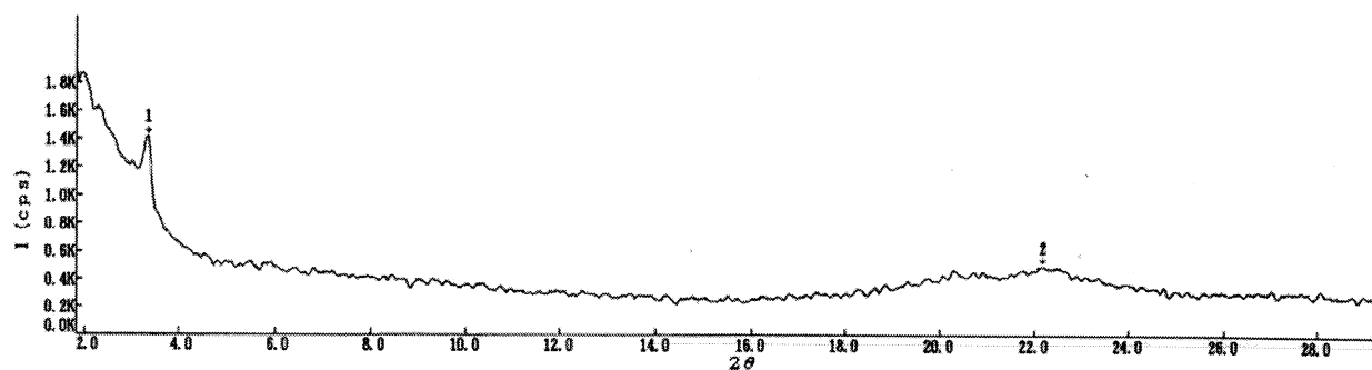
Figure 6. XRD pattern of the polymer A-LPMS.
